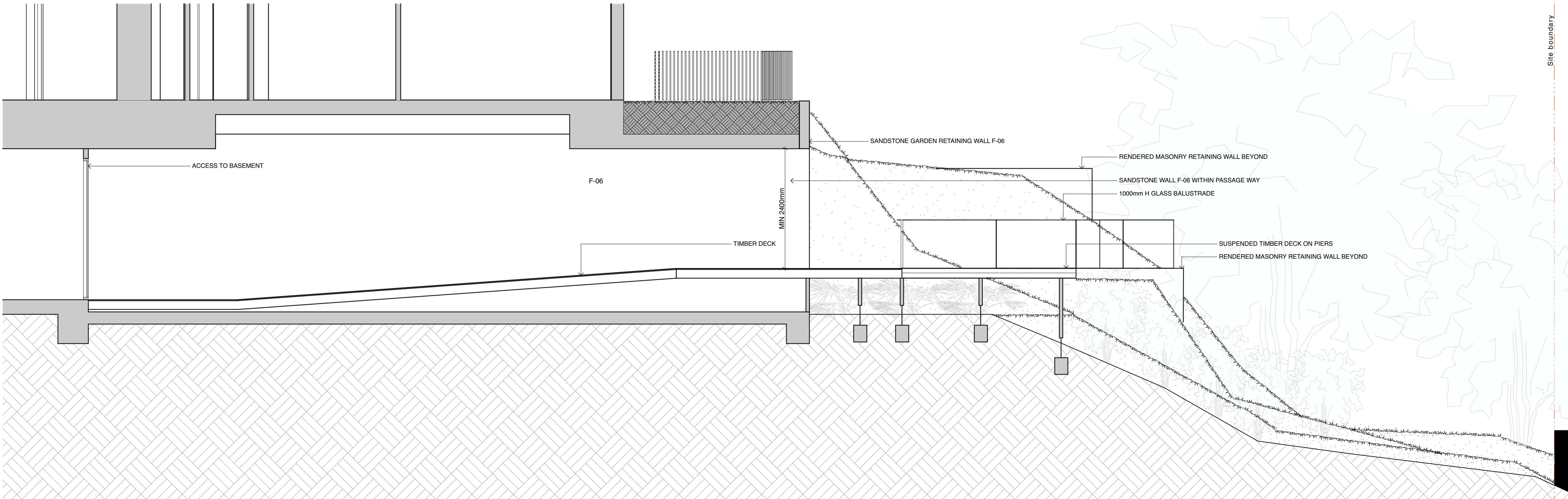
Section H/H
