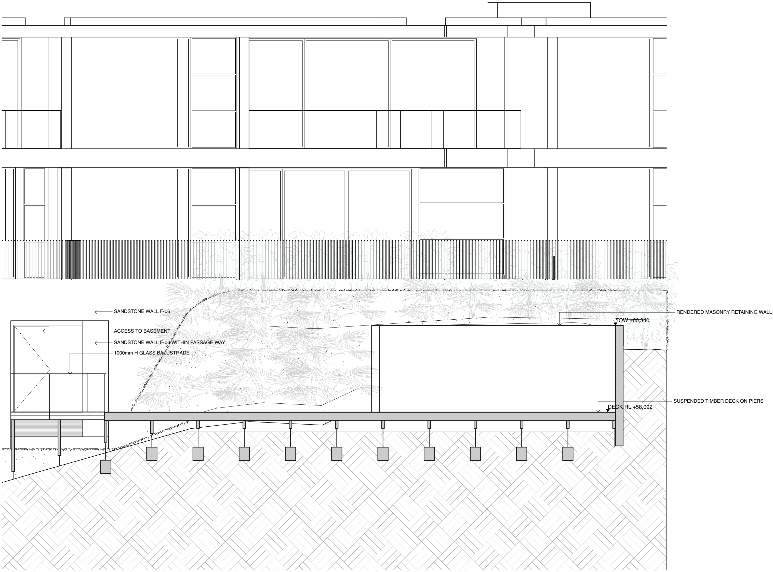
Section G/G
